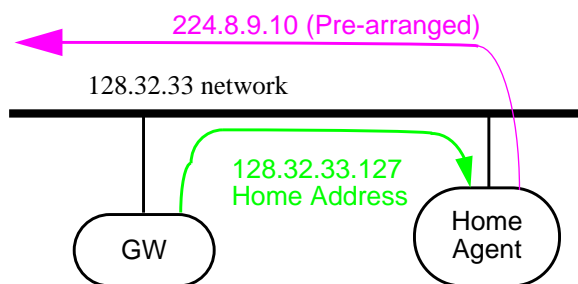
Figure 3. Home Agent Encapsulation.
